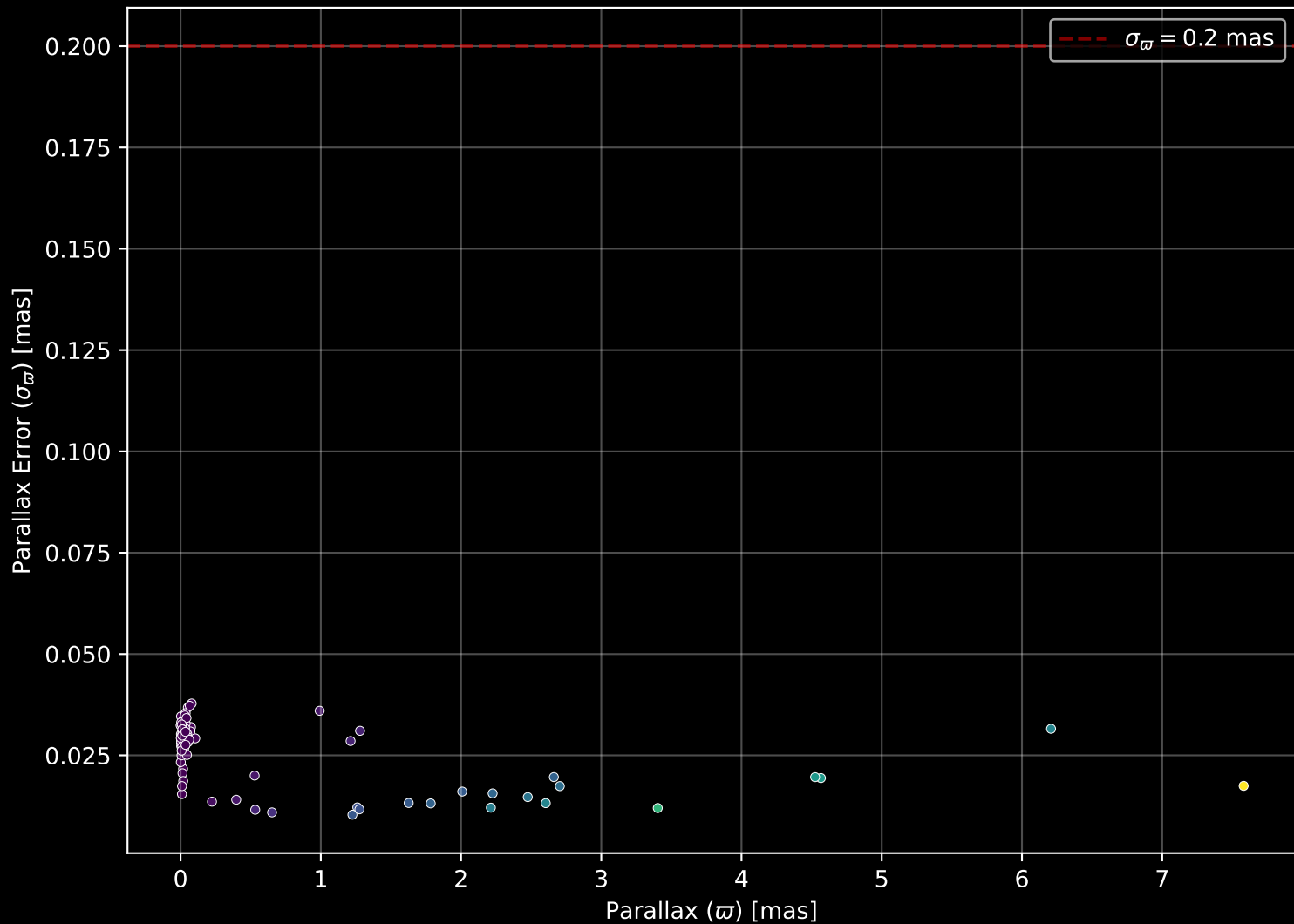
APOGEE DR17 Field: [LMC19] Parallax Quality (n= 95)
