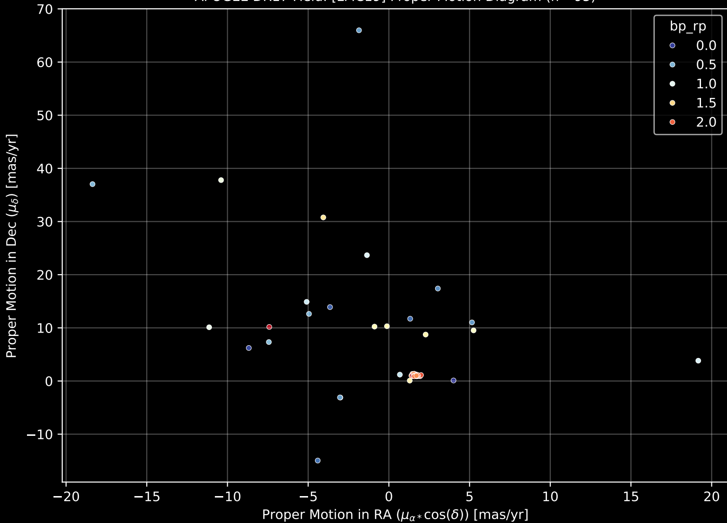
APOGEE DR17 Field: [LMC19] Proper Motion Diagram (n= 95)
