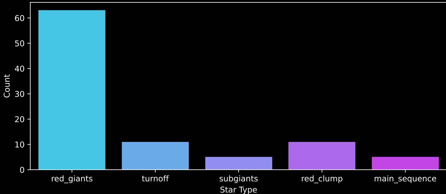
APOGEE DR17 Field: [LMC19] Count plot of Star Type
