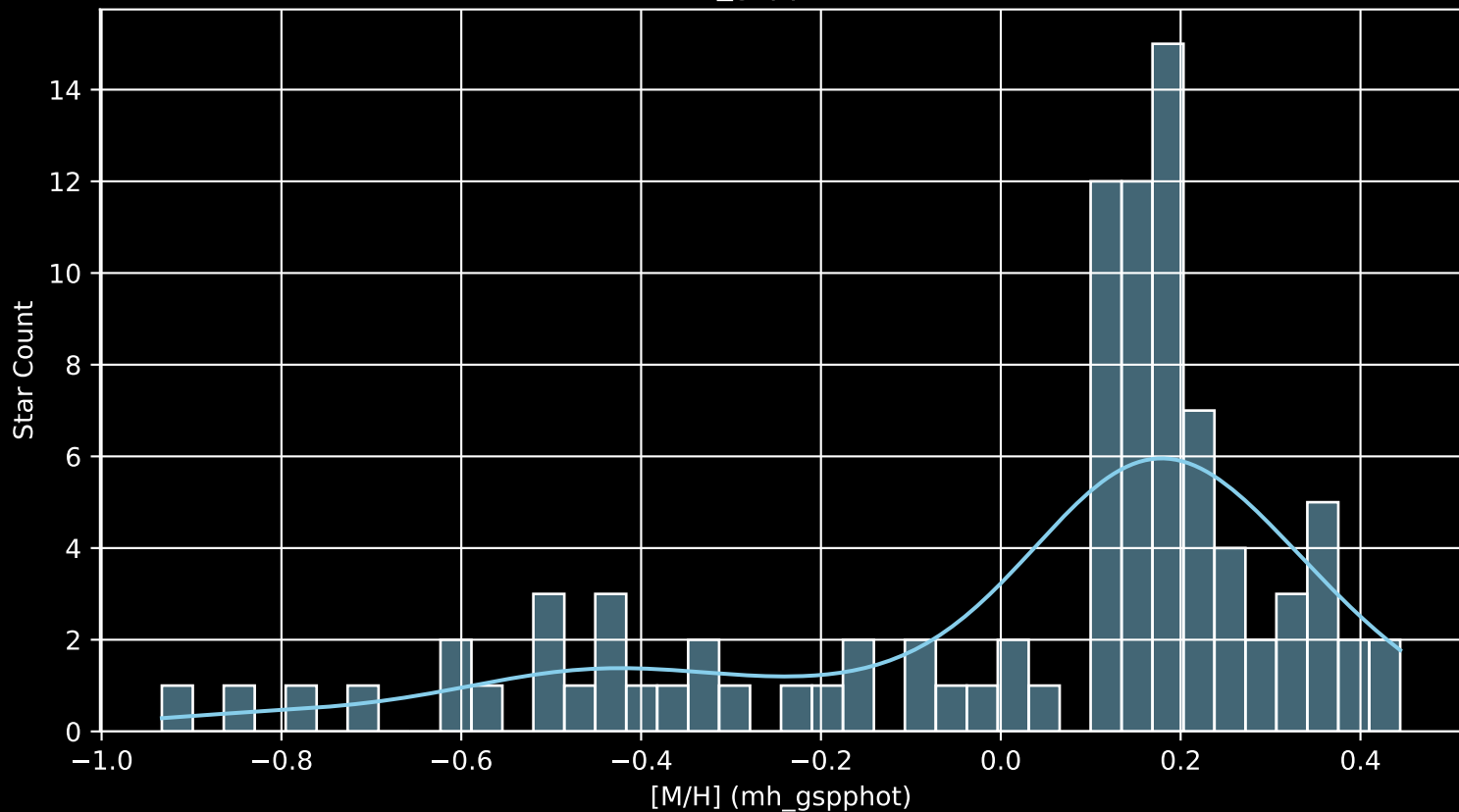
APOGEE DR17 Field: [LMC19 [M/H] (mh_gspphot) (n= 94)
