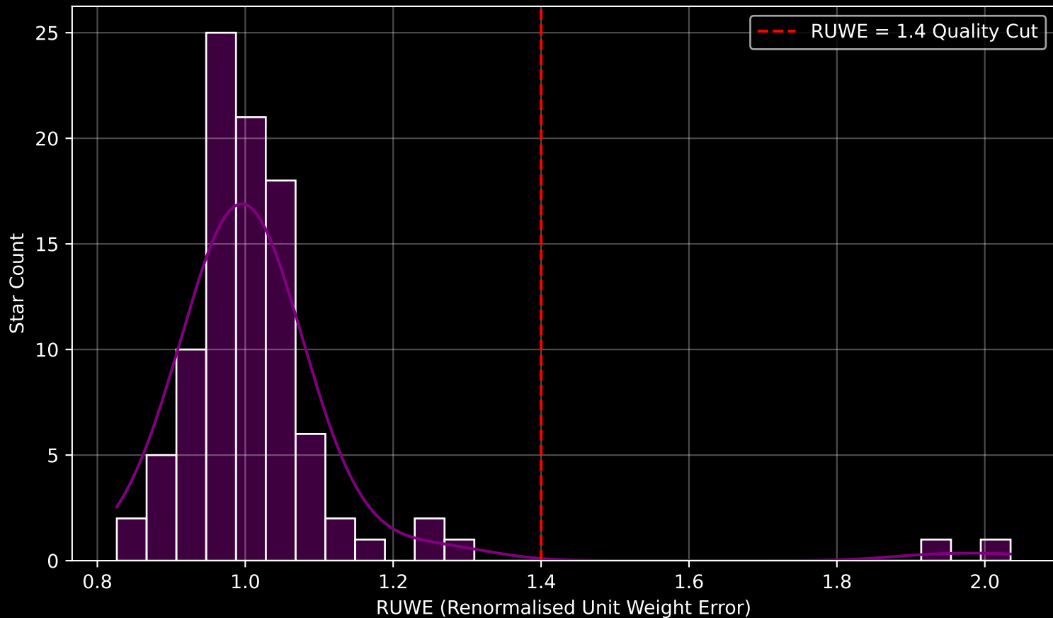
GAPOGEE DR17 Field [LMC19] RUWE Distribution (n= 95)
