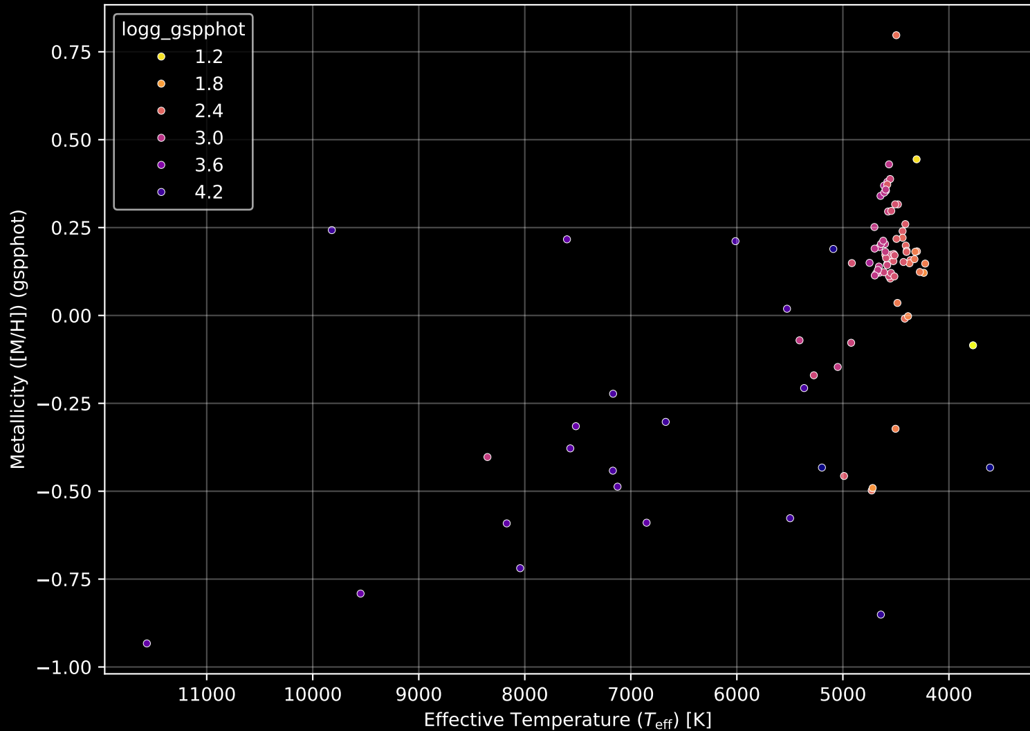
APOGEE DR17 Field: [LMC19] Stellar Population Parameters (n= 95)
