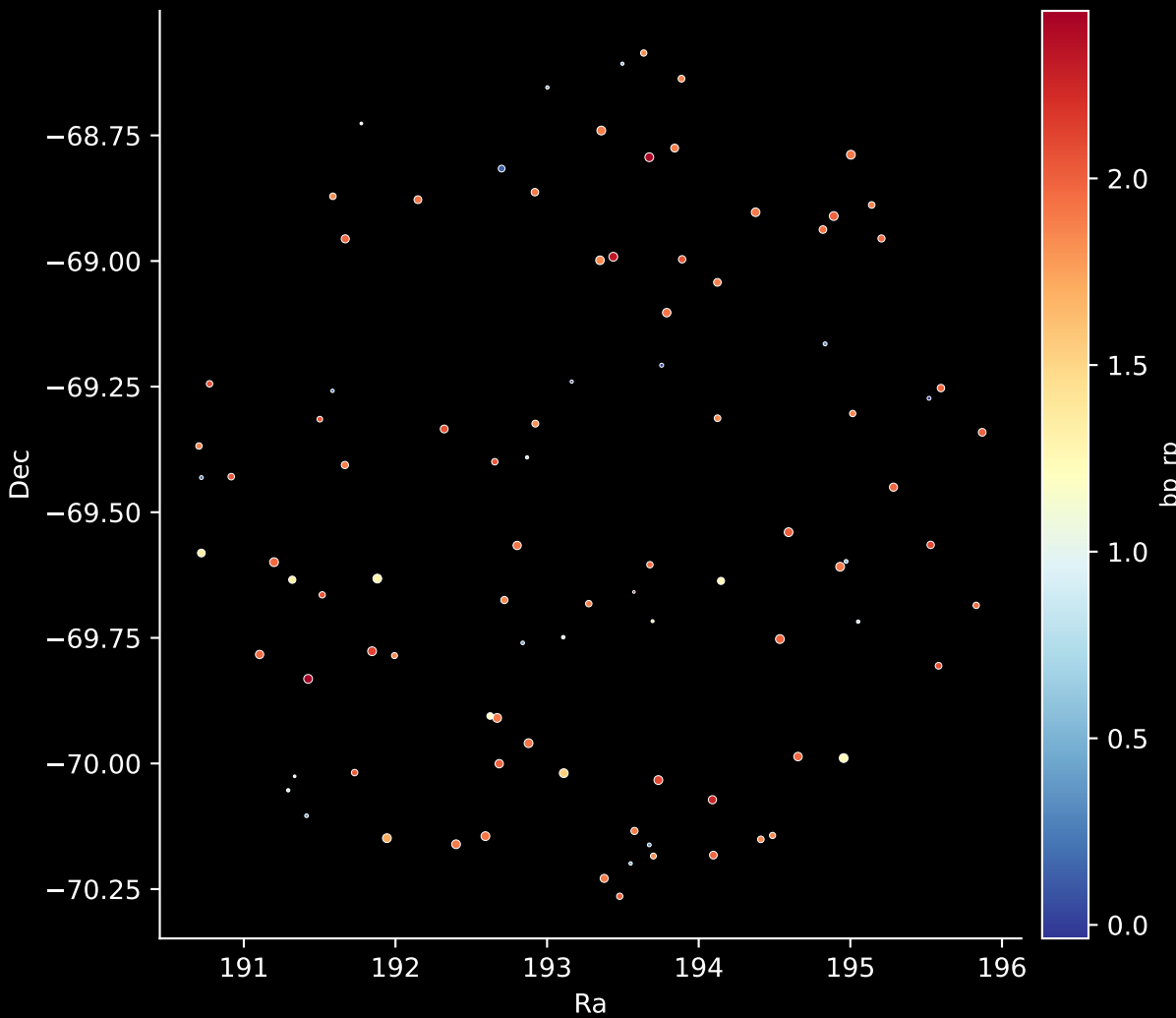
APOGEE DR17 Field: [LMC19] Stars: 95
