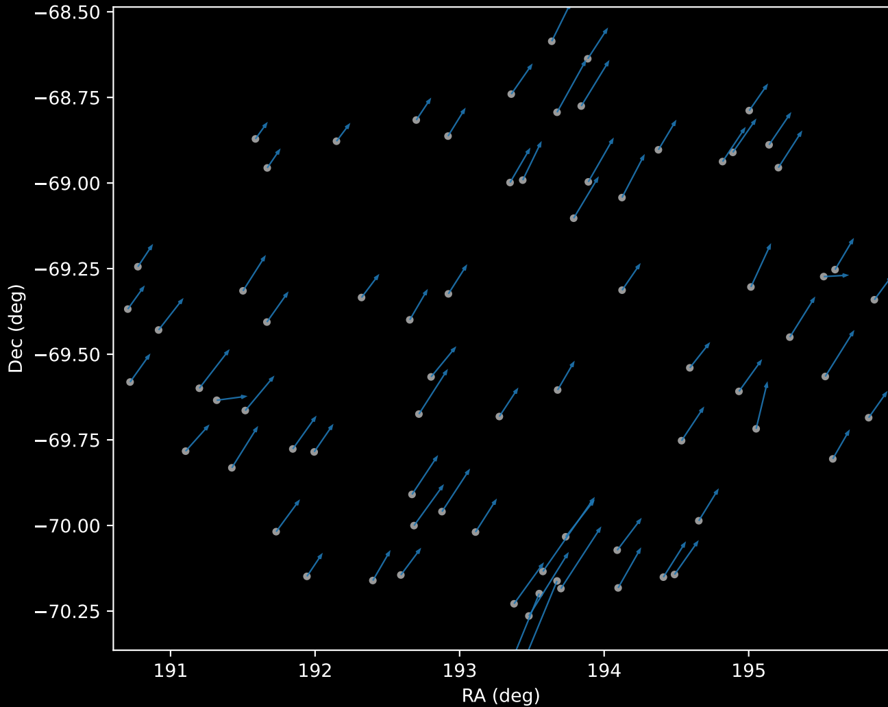
APOGEE DR17 Cluster 0 Proper Motion Vectors (n=74)
